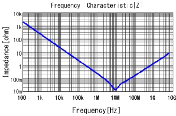
■ GRT155C80J105KE01 |Z| DC0V, 25degC
