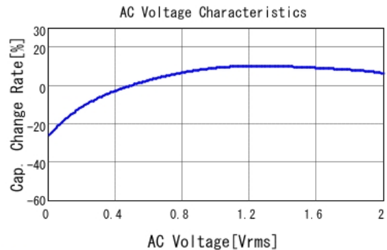
■ GRT155C80J105KE01 C-AC Voltage capchange, DC0V, 25.0d
