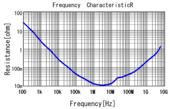
■ GRT155C80J105KE01 R DC0V, 25degC
