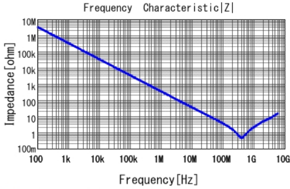
GCM155R72A471KA37 |Z| DCOV, 25degC
