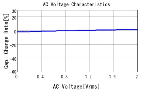
GCM155R72A471KA37 C-AC Voltage capchange, DCOV, 25.0d
