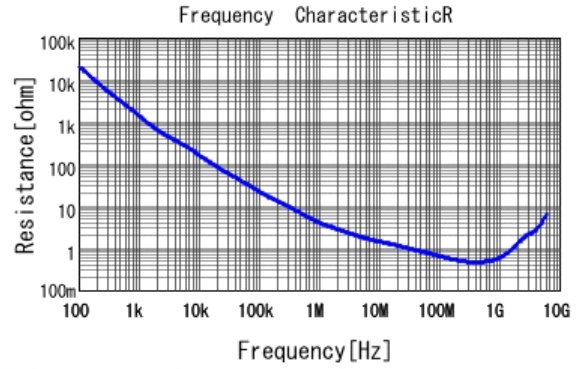
GCM155R72A471KA37 R DCOV, 25degC
