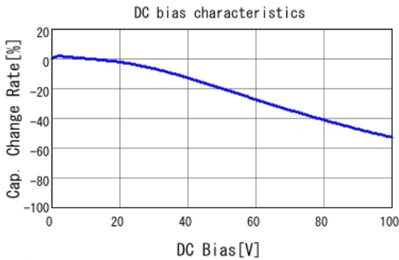
GCM155R72A471KA37 C-DC bias capchange, 25.0degC, AC1.
