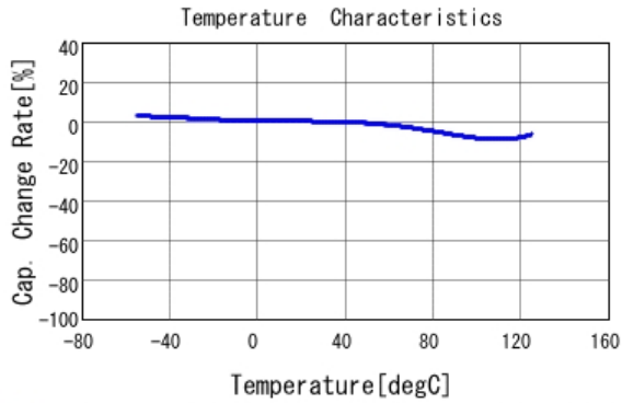
■ GCM155R72A152KA37 C-Temp. capchange, DC0.0V, AC1.0V rm
