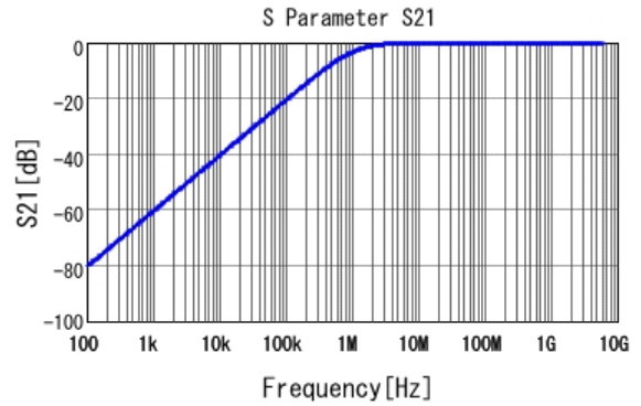
■ GCM155R72A152KA37 S21 DC0V, 25degC
