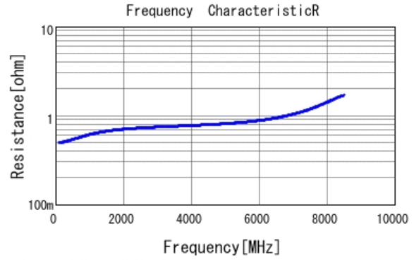
■ GCM1555C1H1R0BA16 R DCOV, 25degC
