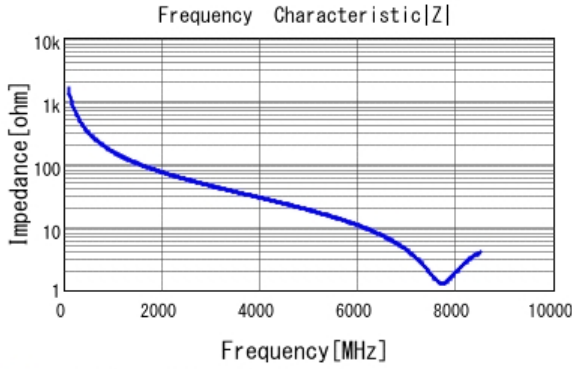
■ GCM1555C1H1R0BA16 |Z| DCOV, 25degC
