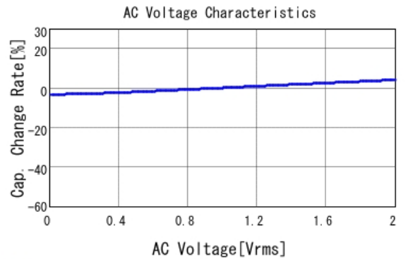
■ GCJ188R92A472KA01 C-AC Voltage capchange, DCOV, 25.0d
