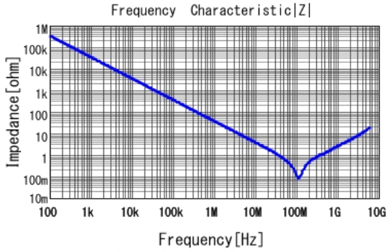
■ GCJ188R92A472KA01 |Z| DCOV, 25degC
