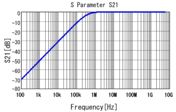
■ GCJ188R92A472KA01 S21 DC0V, 25degC
