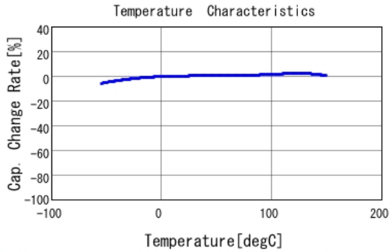
■ GCJ188R92A472KA01 C-Temp. capchange, DC0.0V, AC1.0Vrm
