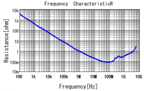
■ GCJ188R92A472KA01 R DCOV, 25degC
