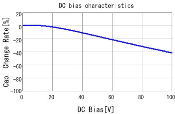
■ GCJ188R92A472KA01 C-DC bias capchange, 25.0degC, AC1.
