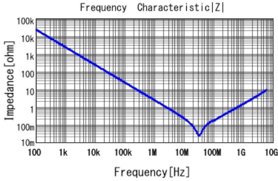
GCM155R71H683KE02 |Z| DCOV, 25degC
