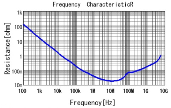
GCM155R71H683KE02 R DCOV, 25degC
