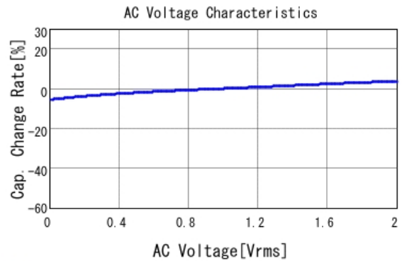
GCM155R71H683KE02 C-AC Voltage capchange, DCOV, 25.0d
