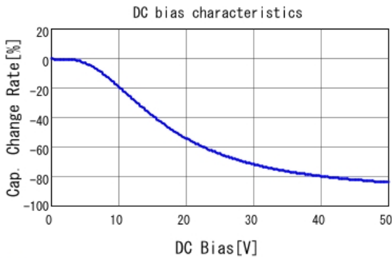
GCM155R71H683KE02 C-DC bias capchange, 25.0degC, AC1.
