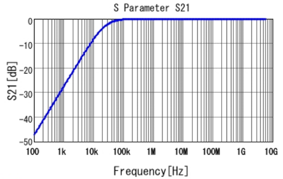
■ GCM155R71H683KE02 S21 DC0V, 25degC
