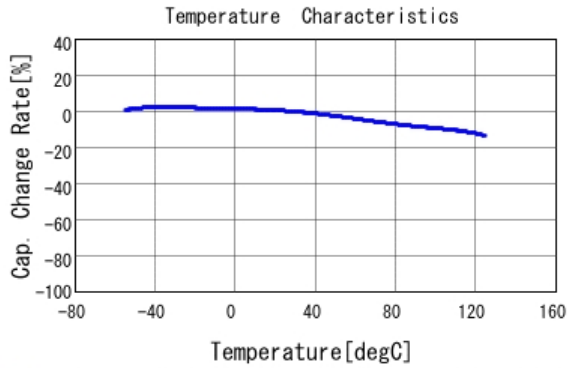
■ GCM155R71H683KE02 C-Temp. capchange, DC0.0V, AC1.0V rm
