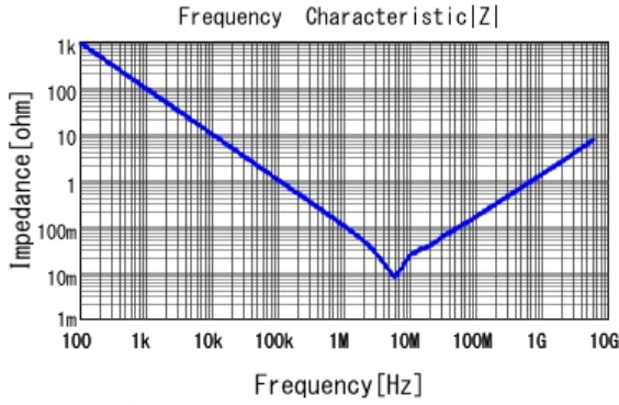
■ GRM155C81E225KE11 |Z| DCOV, 25degC
