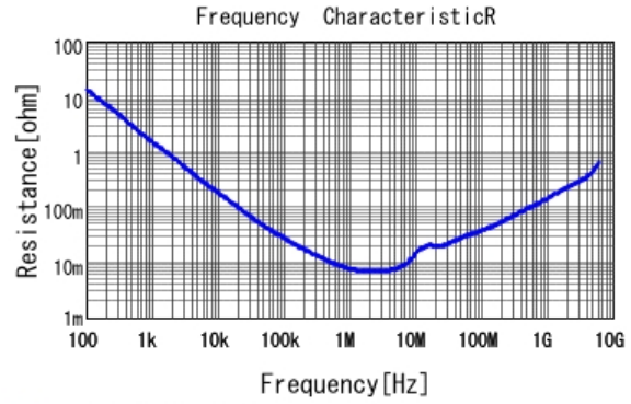
■ GRM155C81E225KE11 R DCOV, 25degC
