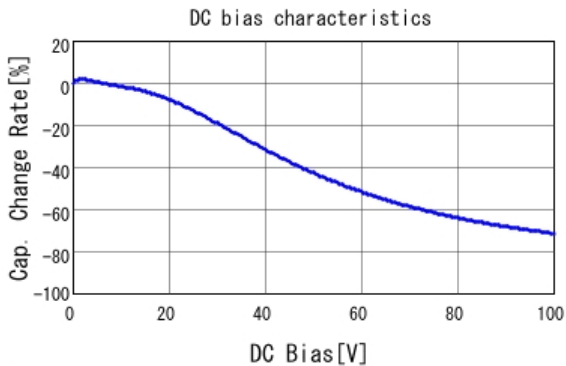
GCM155R72A222KA37 C-DC bias capchange, 25.0degC, AC1.
