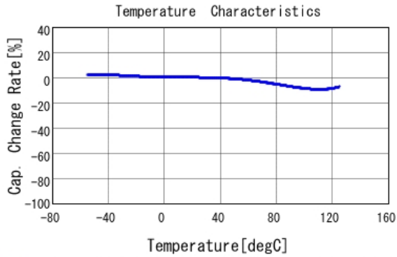
■ GCM155R72A222KA37 C-Temp. capchange, DC0.0V, AC1.0Vrm
