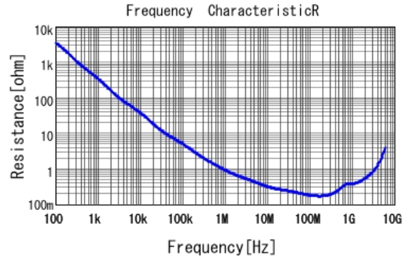
GCM155R72A222KA37 R DCOV, 25degC
