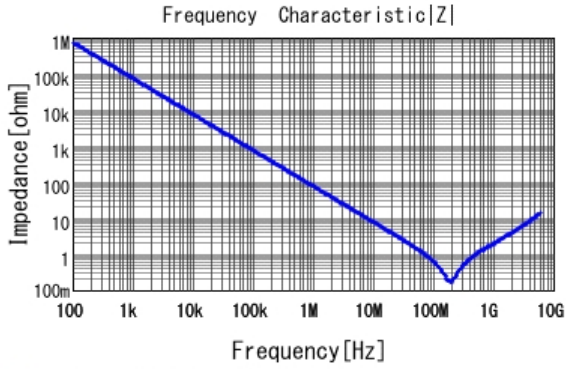
GCM155R72A222KA37 |Z| DCOV, 25degC
