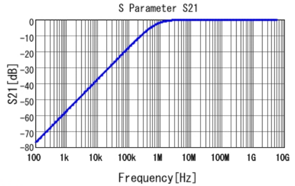
■ GCM155R72A222KA37 S21 DC0V, 25degC
