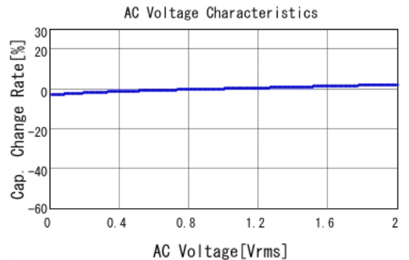
GCM155R72A222KA37 C-AC Voltage capchange, DCOV, 25.0d
