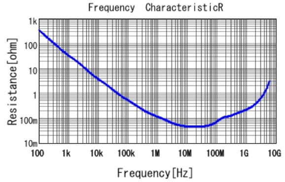
■ GRM155R71E223KA61 R DCOV, 25degC
