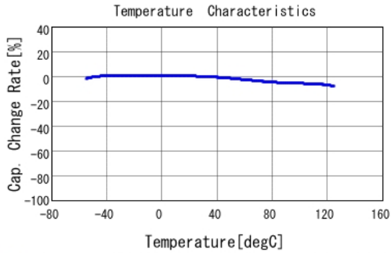
■ GCE188R71H153KA01 C-Temp. capchange, DC0.0V, AC1.0Vrm
