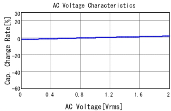
■ GCE188R71H153KA01 C-AC Voltage capchange, DCOV, 25.0d
