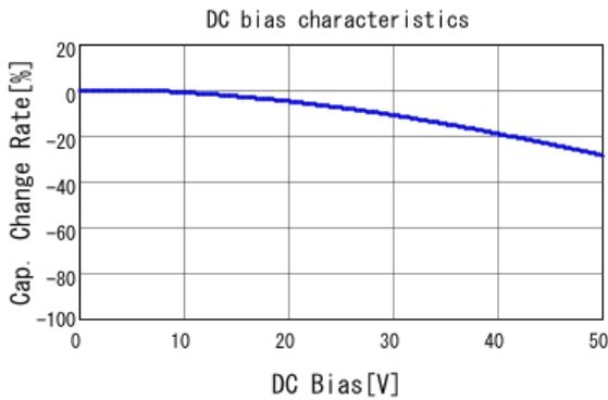
■ GCE188R71H153KA01 C-DC bias capchange, 25.0degC, AC1.
