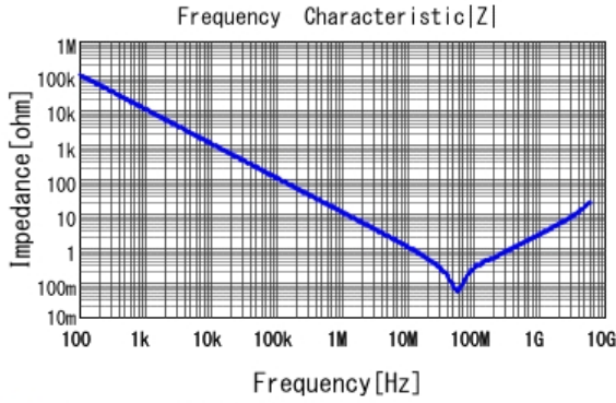
■ GCE188R71H153KA01 |Z| DCOV, 25degC
