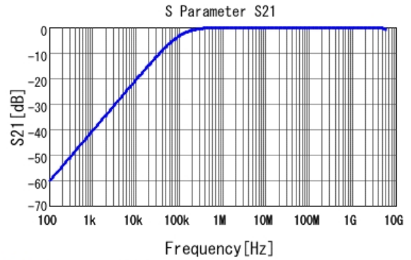
■ GCE188R71H153KA01 S21 DC0V, 25degC
