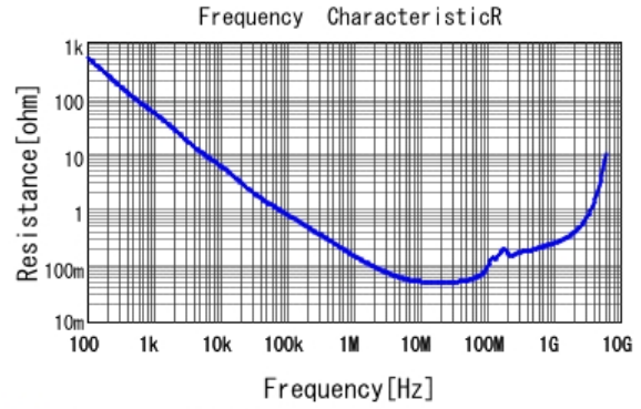
■ GCE188R71H153KA01 R DCOV, 25degC
