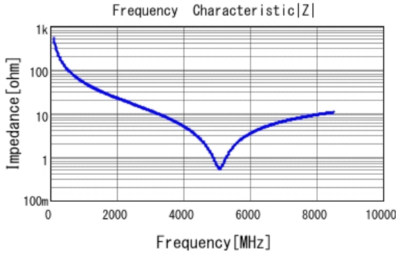
GCM1555C1H3R0BA16 |Z| DCOV, 25degC
