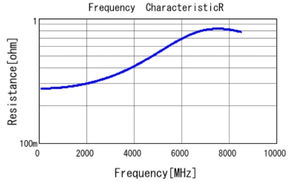
GCM1555C1H3R0BA16 R DCOV, 25degC
