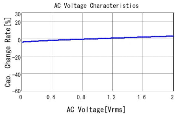
GCM155R71H153KA55 C-AC Voltage capchange, DCOV, 25.0d
