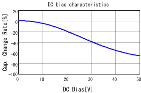
GCM155R71H153KA55 C-DC bias capchange, 25.0degC, AC1.
