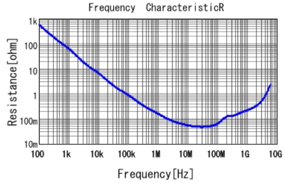
GCM155R71H153KA55 R DCOV, 25degC
