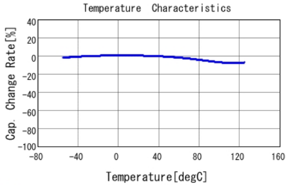
■ GCM155R71H153KA55 C-Temp. capchange, DC0.0V, AC1.0Vrm
