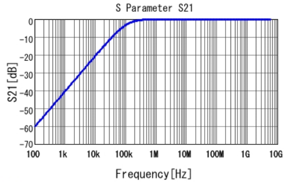
■ GCM155R71H153KA55 S21 DC0V, 25degC
