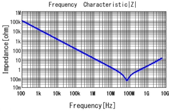
GCM155R71H153KA55 |Z| DCOV, 25degC
