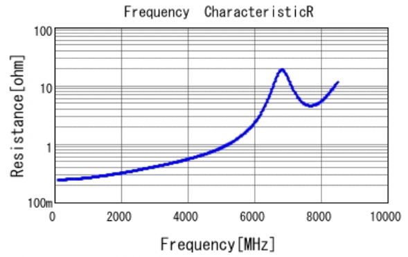
■ GCM1885C2A4R7BA16 R DC0V, 25degC
