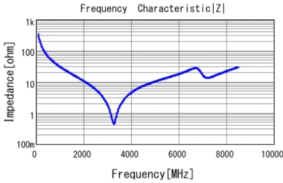
■ GCM1885C2A4R7BA16 |Z| DC0V, 25degC
