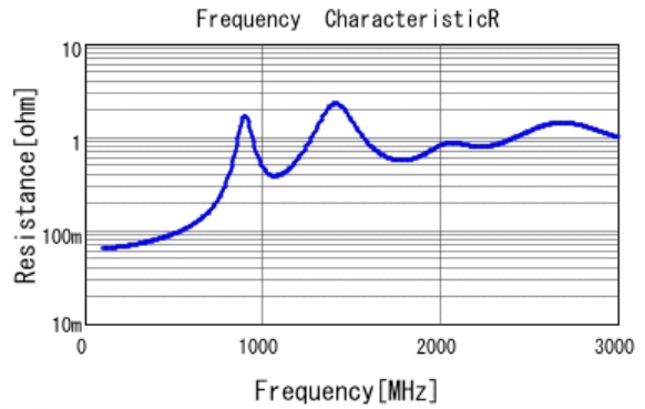
■ GRM21A5C2E331JW01 R DC0V, 25degC
