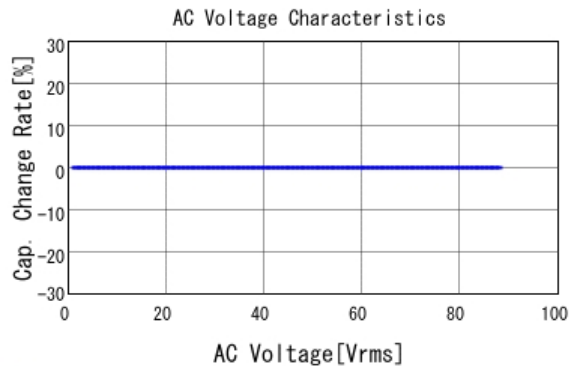
■ GRM21A5C2E331JW01 C-AC Voltage capchange, DC0V, 25.0d
