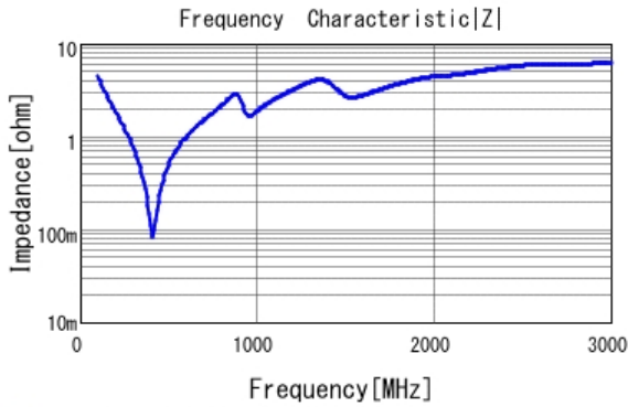
■ GRM21A5C2E331JW01 |Z| DC0V, 25degC
