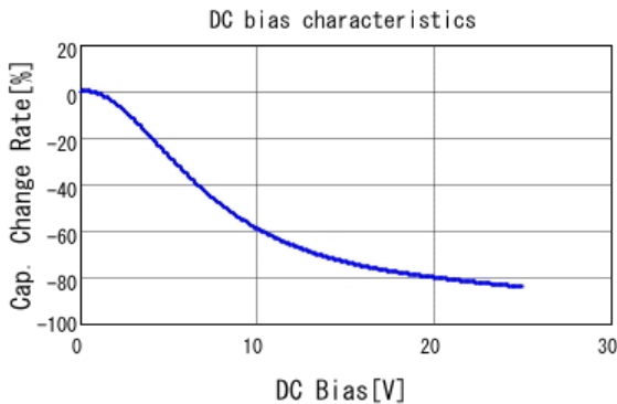
■ GRM188C81E225KE11 C-DC bias capchange, 25.0degC, AC1V
