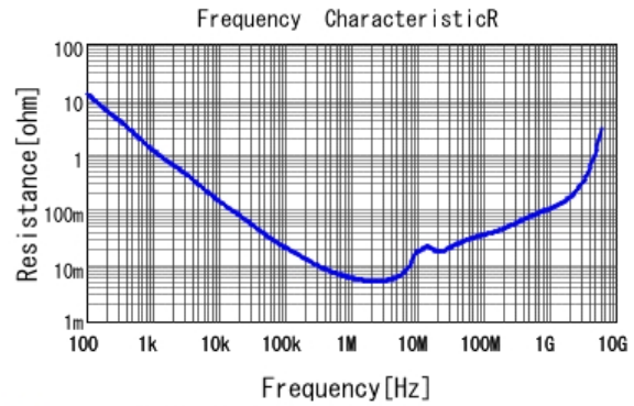
■ GRM188C81E225KE11 R DCOV, 25degC
