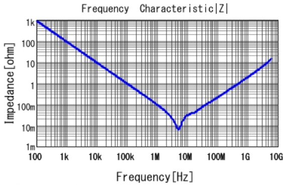
■ GRM188C81E225KE11 |Z| DCOV, 25degC
