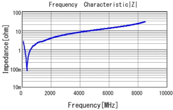
■ GRM1555C1H561GA01 |Z| DCOV, 25degC
