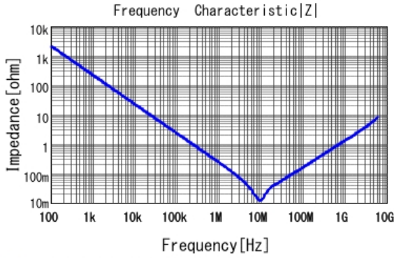
■ GRM155C81C105KE11 |Z| DCOV, 25degC
