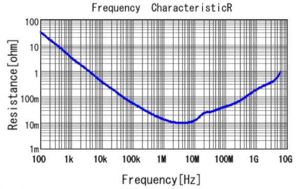
■ GRM155C81C105KE11 R DCOV, 25degC
