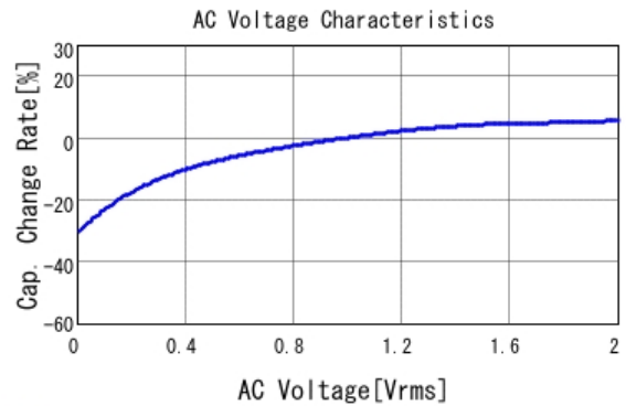
■ GRM155C81C105KE11 C-AC Voltage capchange, DCOV, 25.0d
