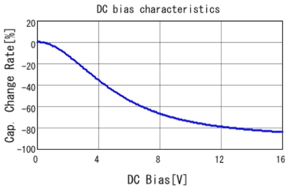
■ GRM155C81C105KE11 C-DC bias capchange, 25.0degC, AC1V
