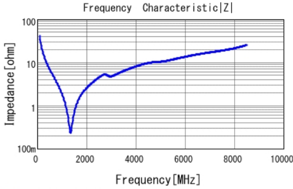
■ GCM1555C1H390JA16 |Z| DCOV, 25degC
