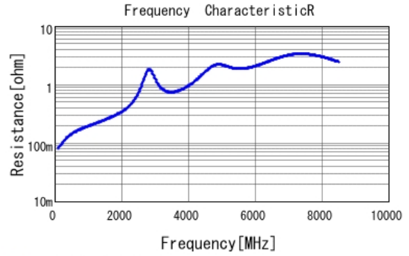
■ GCM1555C1H390JA16 R DCOV, 25degC
