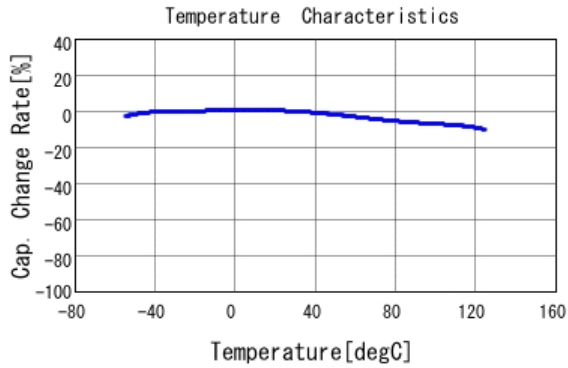
■ GCD188R71H153KA01 C-Temp. capchange, DC0.0V, AC1.0Vrm
