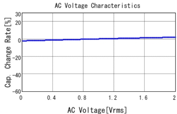
■ GCD188R71H153KA01 C-AC Voltage capchange, DCOV, 25.0d
