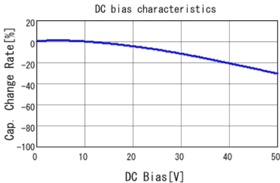
■ GCD188R71H153KA01 C-DC bias capchange, 25.0degC, AC1.
