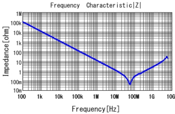
■ GCD188R71H153KA01 |Z| DCOV, 25degC
