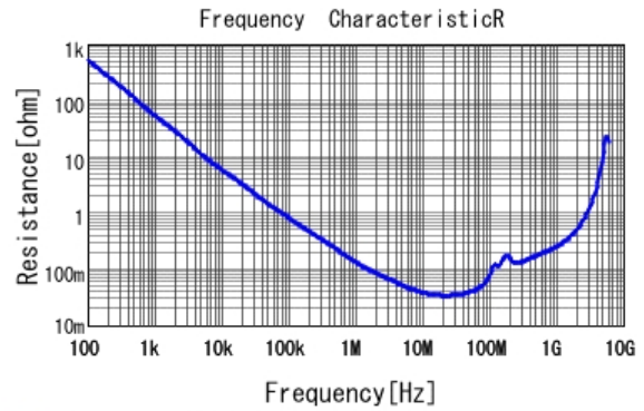
■ GCD188R71H153KA01 R DCOV, 25degC
