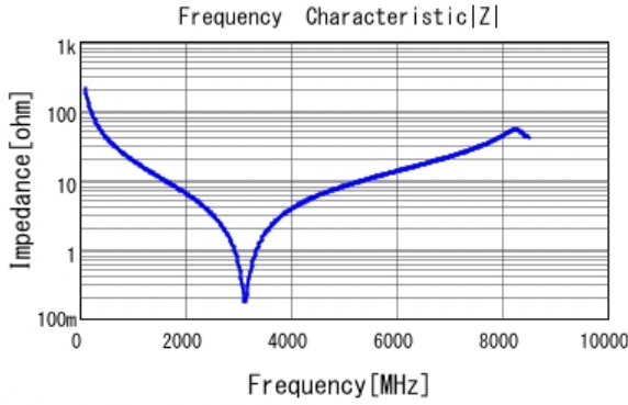
■ GJM1555C1H7R5DB01 |Z| DC0V, 25degC
