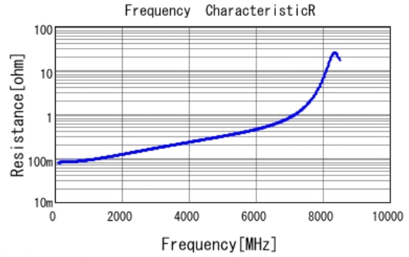
■ GJM1555C1H7R5DB01 R DC0V, 25degC
