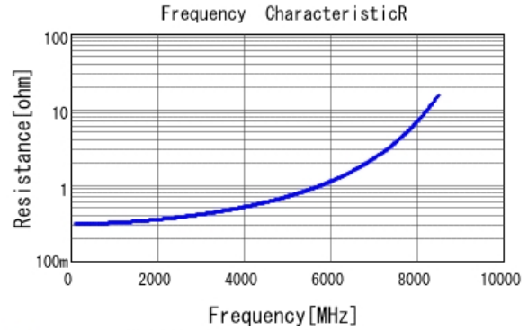
GCM1885C2A2R7BA16 R DC0V, 25degC
