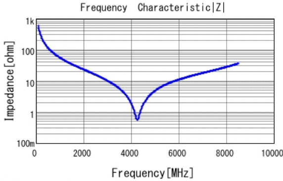
GCM1885C2A2R7BA16 |Z| DC0V, 25degC
