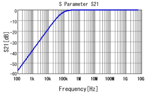
■ GCM155R71E223KA55 S21 DC0V, 25degC
