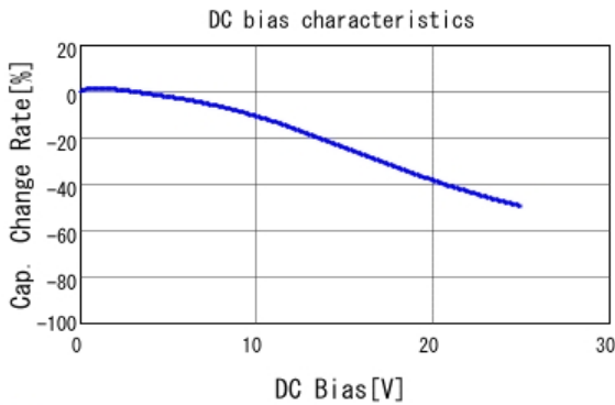
GCM155R71E223KA55 C-DC bias capchange, 25.0degC, AC1.
