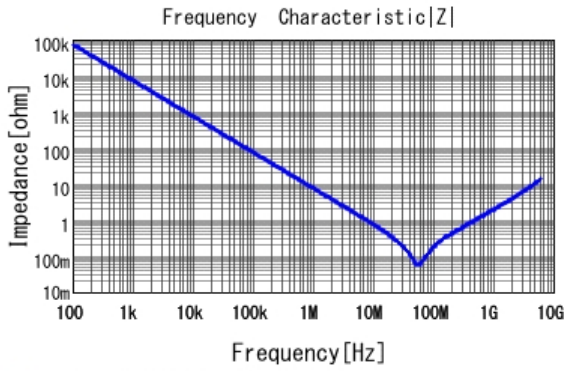
GCM155R71E223KA55 |Z| DCOV, 25degC
