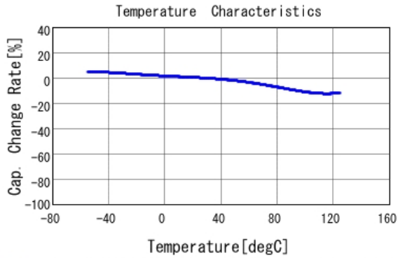
■ GCM155R71E223KA55 C-Temp. capchange, DC0.0V, AC1.0V rm
