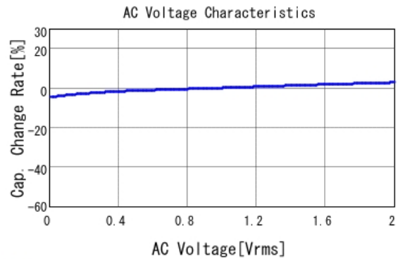
GCM155R71E223KA55 C-AC Voltage capchange, DCOV, 25.0d
