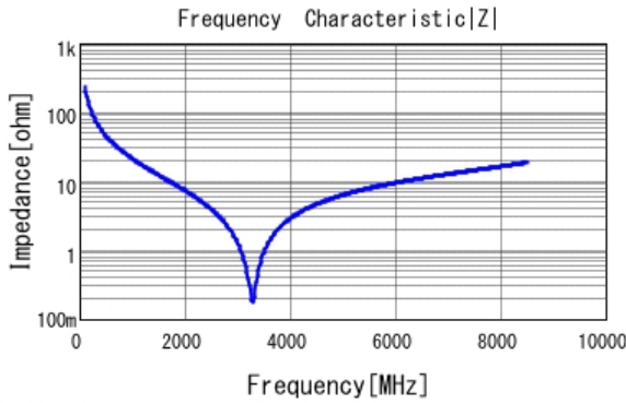
■ GJM1555C1H6R8DB01 |Z| DCOV, 25degC
