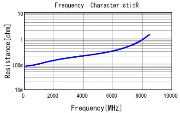
■ GJM1555C1H6R8DB01 R DCOV, 25degC
