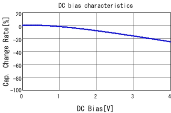
■ GRM155C80G474KE01 C-DC bias capchange, 25.0degC, AC0.
