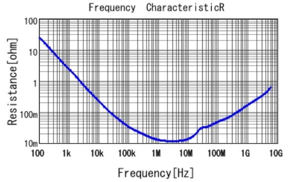
■ GRM155C80G474KE01 R DCOV, 25degC
