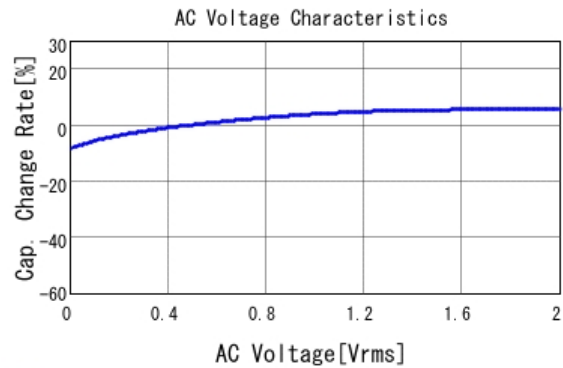
■ GRM155C80G474KE01 C-AC Voltage capchange, DCOV, 25.0d
