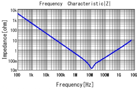
■ GRM155C80G474KE01 |Z| DCOV, 25degC
