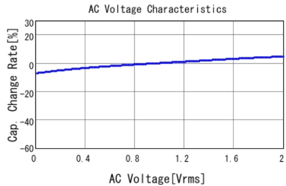
■ GCJ219R71C105KA01 C-AC Voltage capchange, DC0V, 25.0d
