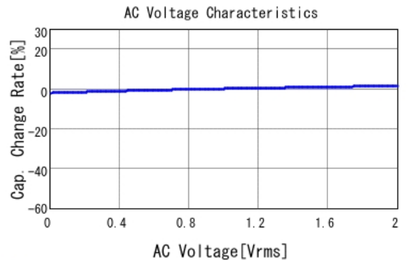
■ GCJ188R72A332KA01 C-AC Voltage capchange, DCOV, 25.0d
