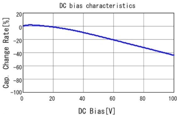
■ GCJ188R72A332KA01 C-DC bias capchange, 25.0degC, AC1.
