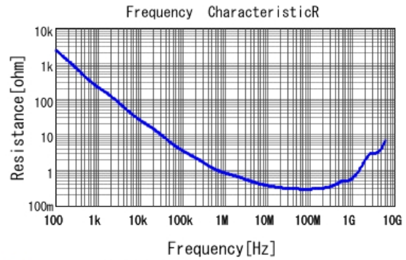
■ GCJ188R72A332KA01 R DCOV, 25degC
