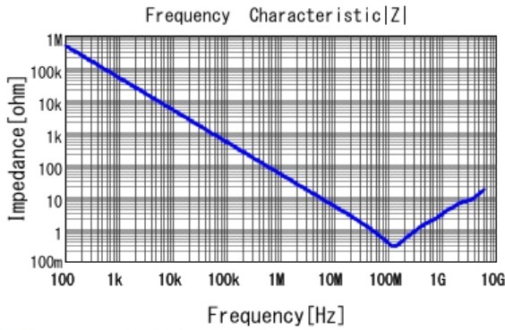
■ GCJ188R72A332KA01 |Z| DCOV, 25degC
