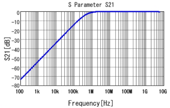
■ GCJ188R72A332KA01 S21 DC0V, 25degC
