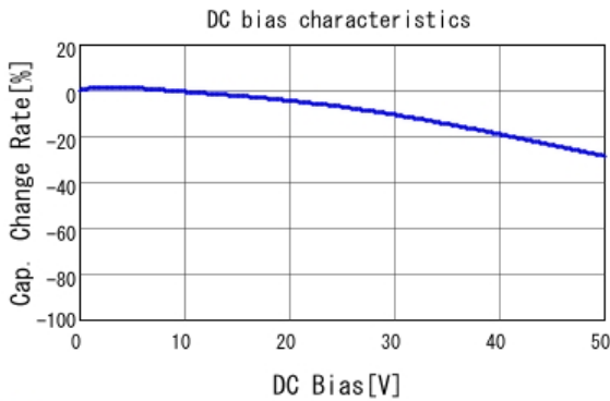
■ GCJ188R71H682KA01 C-DC bias capchange, 25.0degC, AC1.
