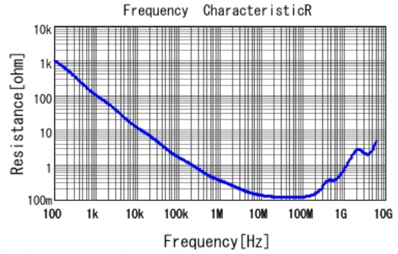
■ GCJ188R71H682KA01 R DCOV, 25degC
