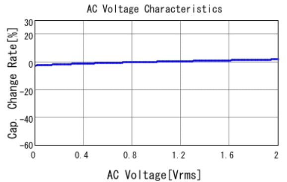
■ GCJ188R71H682KA01 C-AC Voltage capchange, DCOV, 25.0d
