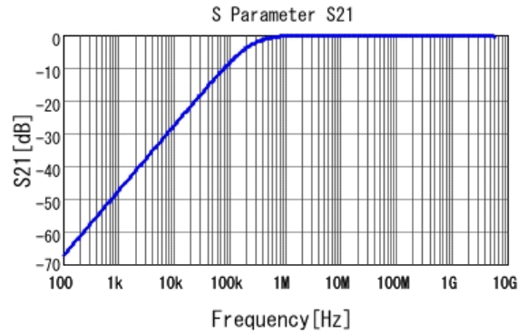
■ GCJ188R71H682KA01 S21 DC0V, 25degC
