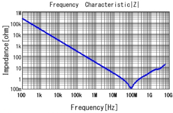
■ GCJ188R71H682KA01 |Z| DCOV, 25degC
