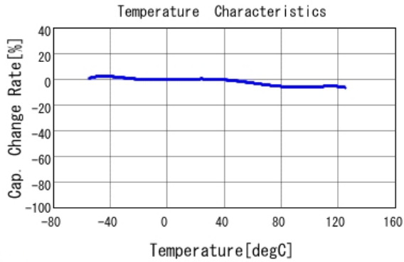
■ GCJ188R71H682KA01 C-Temp. capchange, DC0.0V, AC1.0V rm
