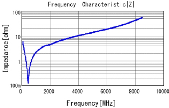
■ GCM1555C1H271JA16 |Z| DCOV, 25degC
