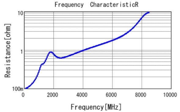
■ GCM1555C1H271JA16 R DCOV, 25degC
