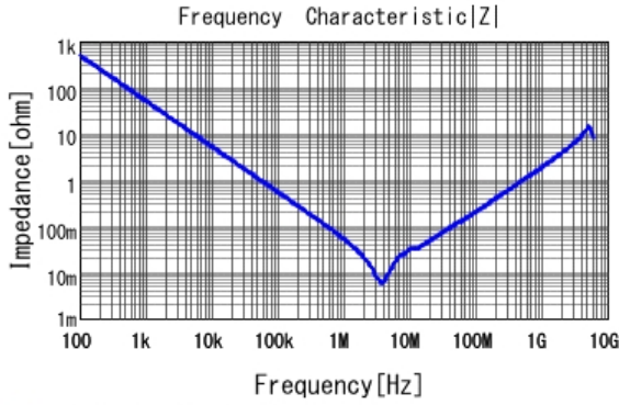
■ GRM219R6YA475KA73 |Z| DCOV, 25degC
