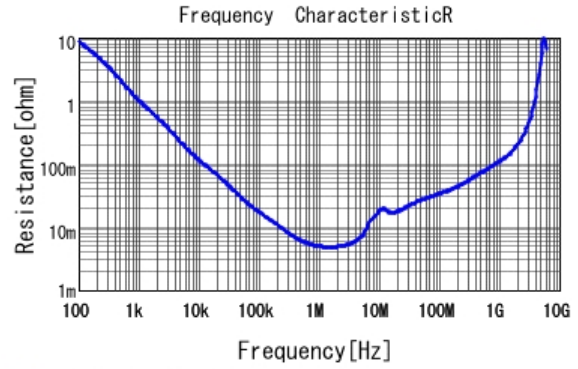
■ GRM219R6YA475KA73 R DCOV, 25degC
