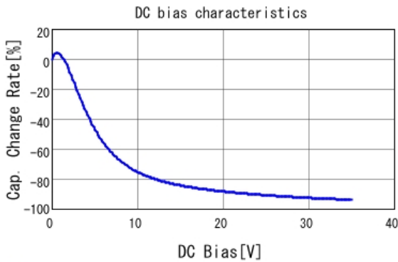
■ GRM219R6YA475KA73 C-DC bias capchange, 25.0degC, AC1.
