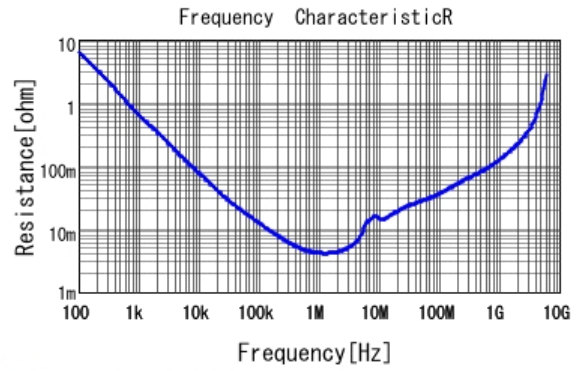
■ GRT188R61C475KE13 R DCOV, 25degC
