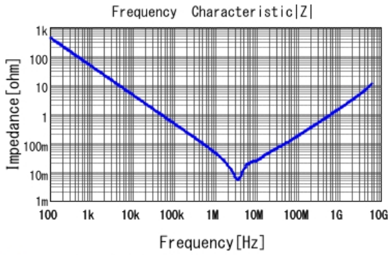
■ GRT188R61C475KE13 |Z| DCOV, 25degC
