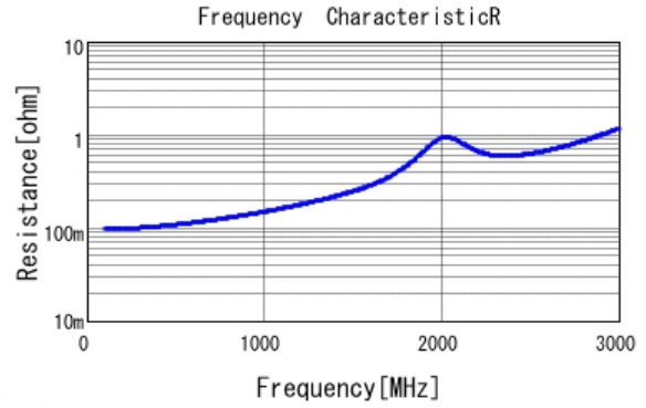
■ GRM21A5C2E121JW01 R DC0V, 25degC
