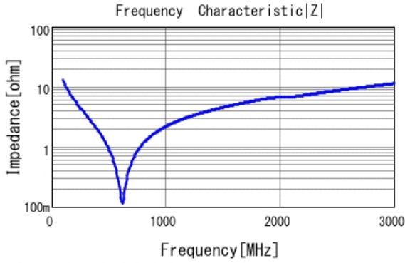
■ GRM21A5C2E121JW01 |Z| DC0V, 25degC
