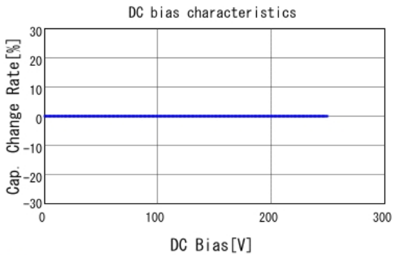
■ GRM21A5C2E121JW01 C-DC bias capchange, 25.0degC, AC1V
