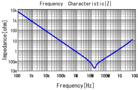
■ GRT155R61E474KE01 |Z| DCOV, 25degC
