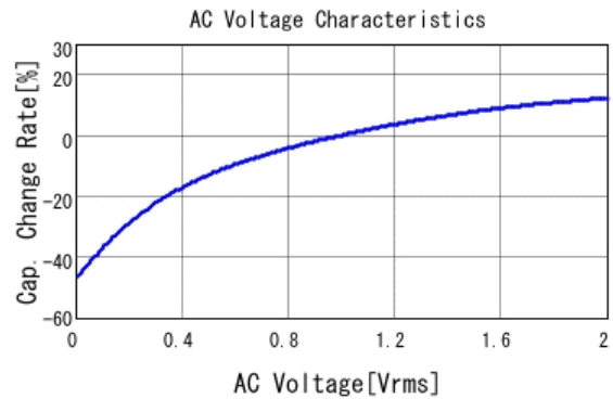
■ GRT155R61E474KE01 C-AC Voltage capchange, DCOV, 25.0d
