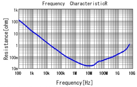
■ GRT155R61E474KE01 R DCOV, 25degC
