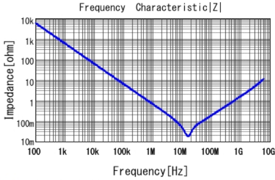
■ GRT155R6YA474KE01 |Z| DCOV, 25degC
