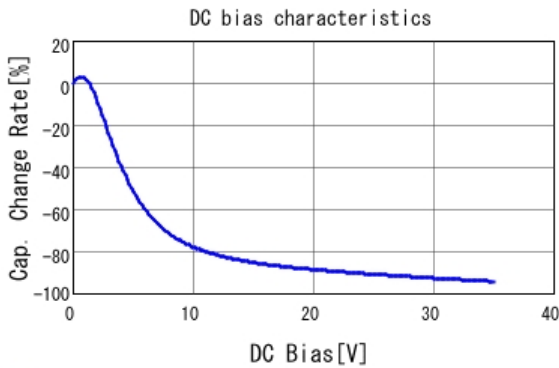
■ GRT155R6YA474KE01 C-DC bias capchange, 25.0degC, AC1.
