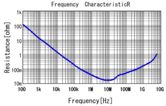
■ GRT155R6YA474KE01 R DCOV, 25degC
