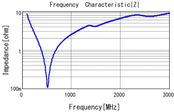
■ GRM21A5C2E181JW01 |Z| DC0V, 25degC
