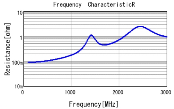
■ GRM21A5C2E181JW01 R DC0V, 25degC
