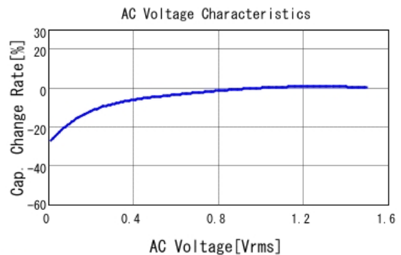
■ GRT188R61C106KE13 C-AC Voltage capchange, DCOV, 25.0d
