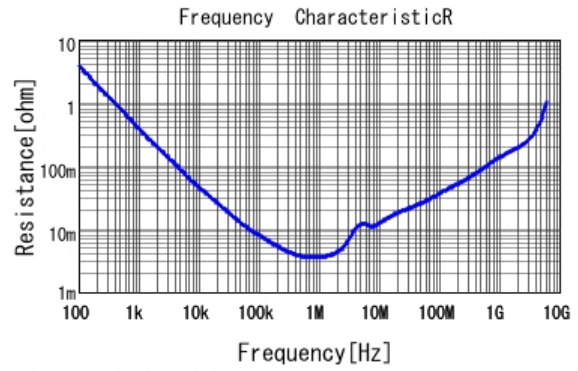
■ GRT188R61C106KE13 R DCOV, 25degC
