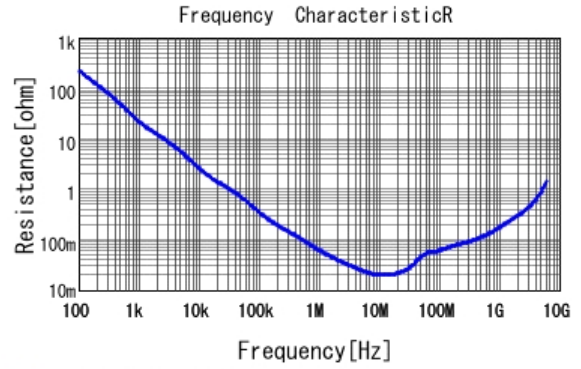
■ GRT155C81E224KE01 R DC0V, 25degC
