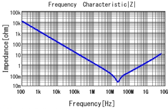
■ GRT155C81E224KE01 |Z| DC0V, 25degC
