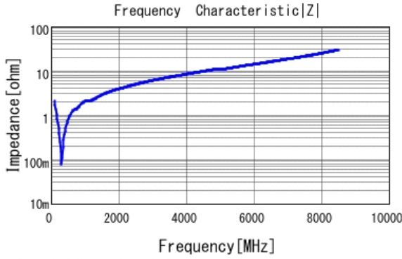
■ GRM1555C1H681GA01 |Z| DCOV, 25degC
