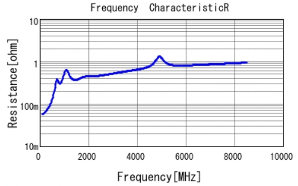
■ GRM1555C1H681GA01 R DCOV, 25degC
