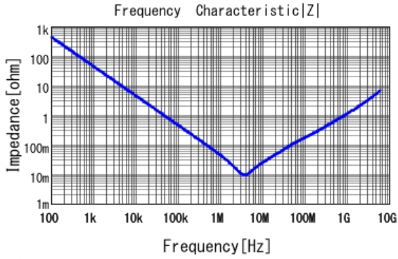
■ GRM153R60G475ME15 |Z| DCOV, 25degC
