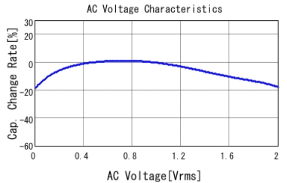
■ GRM153R60G475ME15 C-AC Voltage capchange, DCOV, 25.0d
