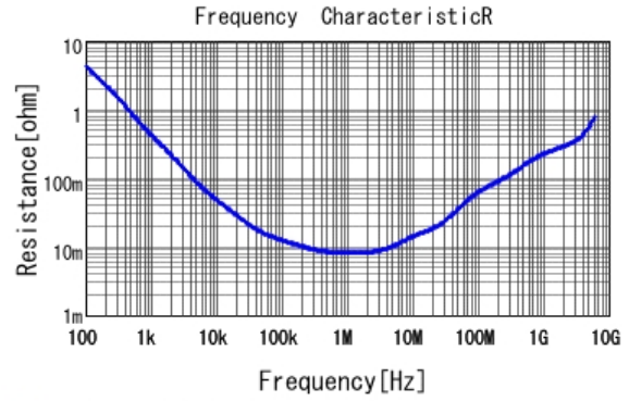
■ GRM153R60G475ME15 R DCOV, 25degC
