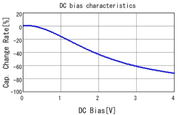
■ GRM153R60G475ME15 C-DC bias capchange, 25.0degC, AC0.
