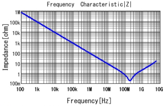
■ GRM155R71H222KA01 |Z| DCOV, 25degC
