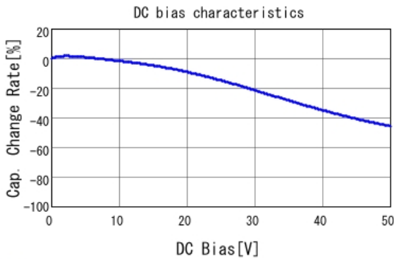
■ GRM155R71H222KA01 C-DC bias capchange, 25.0degC, AC1.
