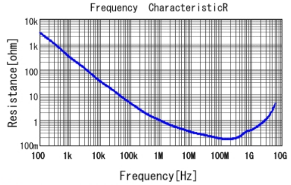
■ GRM155R71H222KA01 R DCOV, 25degC
