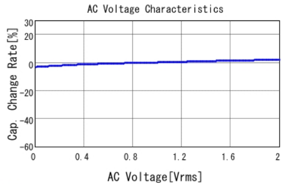
■ GRM155R71H222KA01 C-AC Voltage capchange, DCOV, 25.0d
