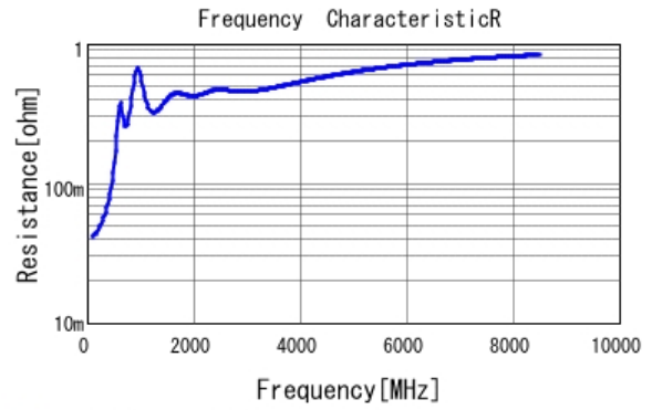
■ GRM1555C1H821JA01 R DCOV, 25degC
