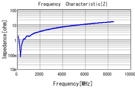
■ GRM1555C1H821JA01 |Z| DCOV, 25degC
