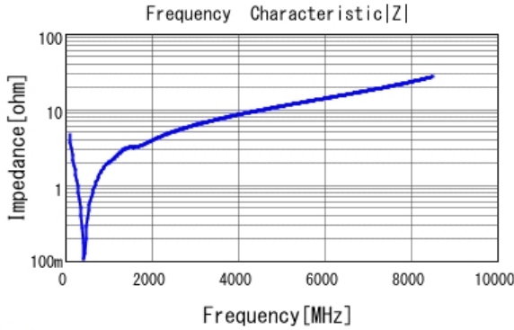
■ GRM1555C1H331GA01 |Z| DCOV, 25degC
