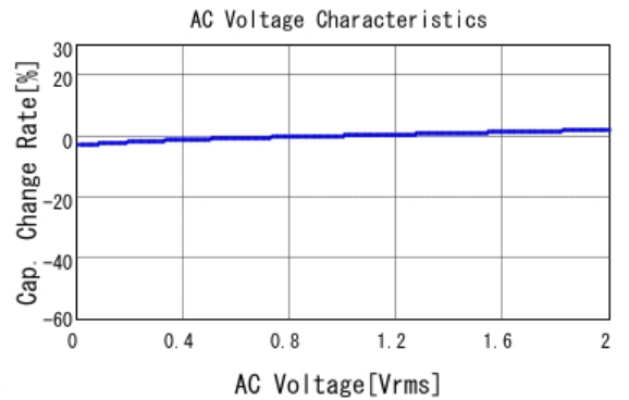
■ GRM155R72A102KA01 C-AC Voltage capchange, DCOV, 25.0d
