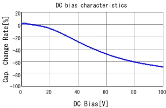
■ GRM155R72A102KA01 C-DC bias capchange, 25.0degC, AC1.
