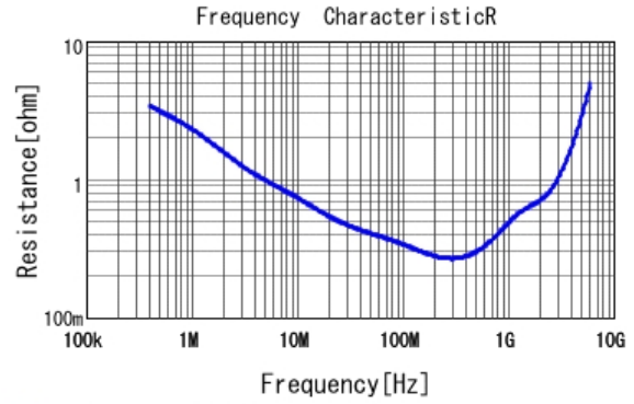
■ GRM155R72A102KA01 R DCOV, 25degC
