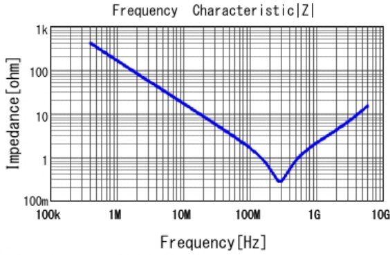
■ GRM155R72A102KA01 |Z| DCOV, 25degC
