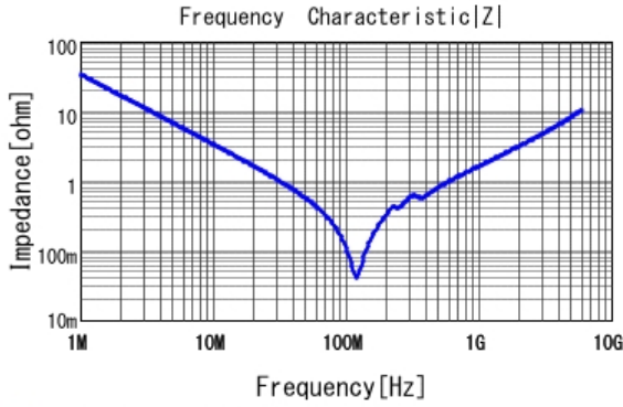
■ GRM1557U1A472JA01 |Z| DCOV, 25degC
