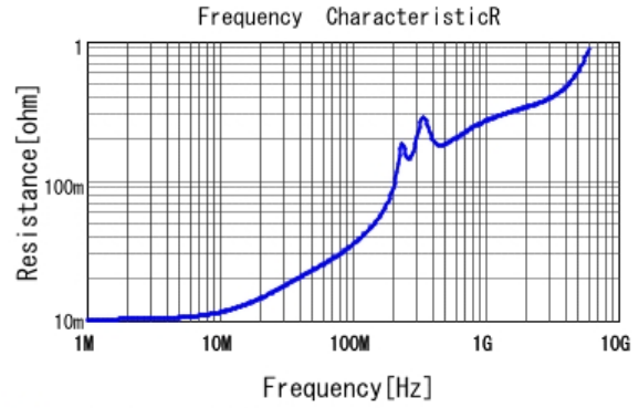
■ GRM1557U1A472JA01 R DCOV, 25degC
