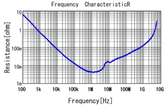
■ GRM188R61C475ME11 R DCOV, 25degC
