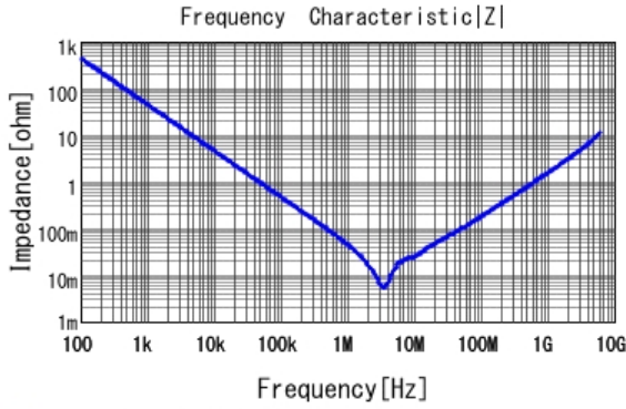
■ GRM188R61C475ME11 |Z| DCOV, 25degC
