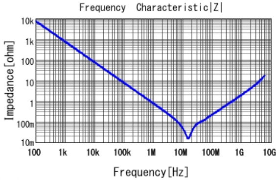
■ GRM188R71E224KA88 |Z| DCOV, 25degC
