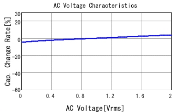
■ GRM188R71E224KA88 C-AC Voltage capchange, DCOV, 25.0d
