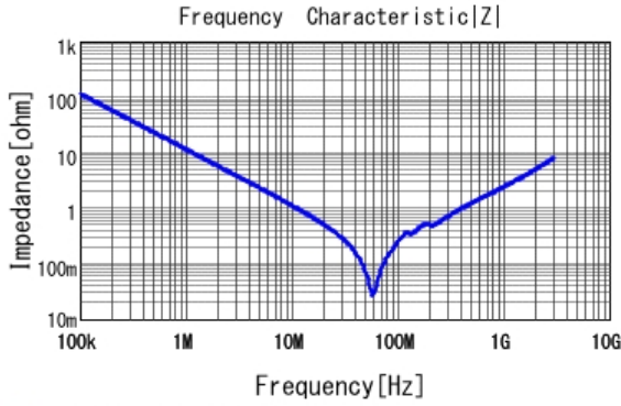
■ GR321AD72E153KW01 |Z| DCOV, 25degC
