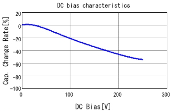
■ GR321AD72E153KW01 C-DC bias capchange, 25.0degC, AC1V
