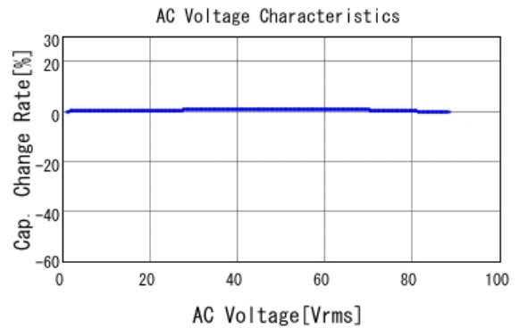
■ GR321AD72E153KW01 C-AC Voltage capchange, DCOV, 25.0d
