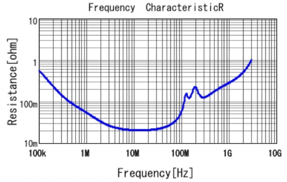
■ GR321AD72E153KW01 R DCOV, 25degC
