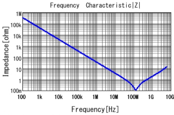
GCM155R71H472KA37 |Z| DCOV, 25degC
