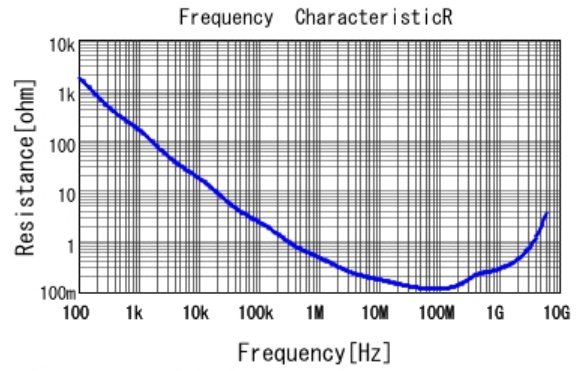
GCM155R71H472KA37 R DCOV, 25degC
