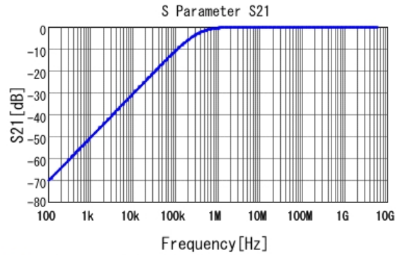
■ GCM155R71H472KA37 S21 DC0V, 25degC
