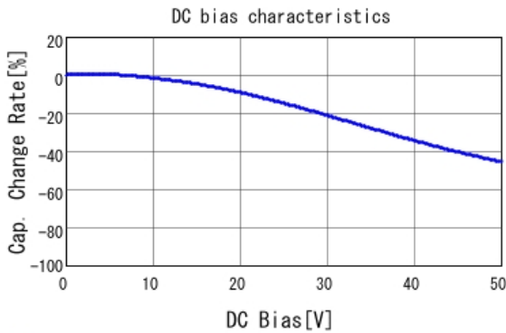
GCM155R71H472KA37 C-DC bias capchange, 25.0degC, AC1.
