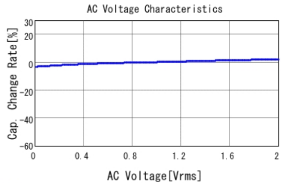
GCM155R71H472KA37 C-AC Voltage capchange, DCOV, 25.0d
