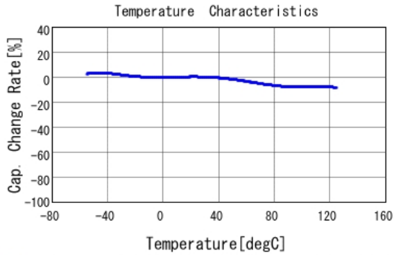
■ GCM155R71H472KA37 C-Temp. capchange, DC0.0V, AC1.0Vrm
