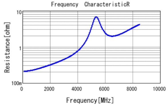
■ GCM1555C1H100FA16 R DCOV, 25degC
