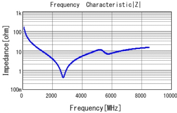
■ GCM1555C1H100FA16 |Z| DCOV, 25degC
