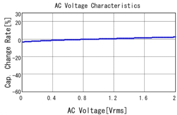
■ GCJ188R71H223KA01 C-AC Voltage capchange, DCOV, 25.0d
