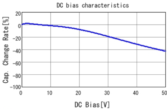
■ GCJ188R71H223KA01 C-DC bias capchange, 25.0degC, AC1.
