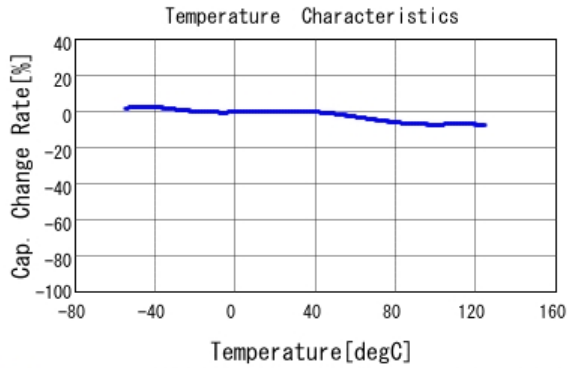
■ GCJ188R71H223KA01 C-Temp. capchange, DC0.0V, AC1.0Vrm
