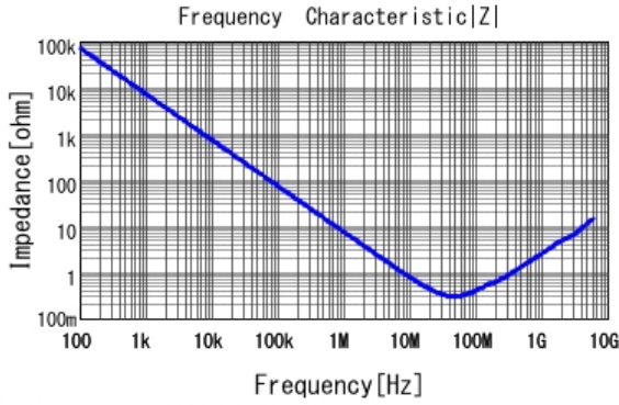
■ GCJ188R71H223KA01 |Z| DCOV, 25degC
