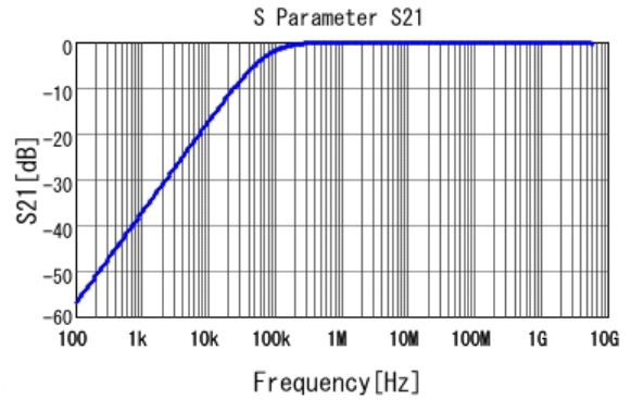
■ GCJ188R71H223KA01 S21 DC0V, 25degC
