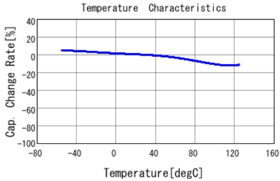
■ GCM155R71E153KA55 C-Temp. capchange, DC0.0V, AC1.0V rm
