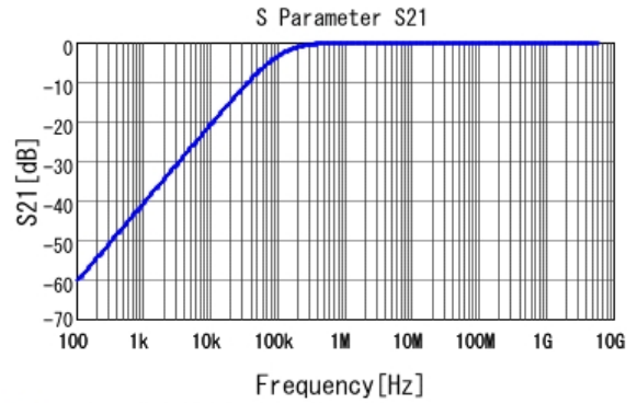
■ GCM155R71E153KA55 S21 DC0V, 25degC
